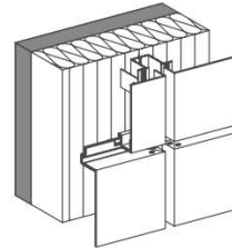
4 GLUED for vertical / horizontal façade structuring
